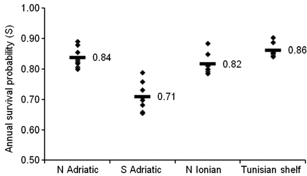
Figure 3. Annual survival probability (S) of loggerhead turtles from four Mediterranean areas, estimated from age distributions obtained through the eight age–size curves available for the Mediterranean Sea and based on capture–mark–recapture (Casale et al. , 2009), length–frequency analysis (Casale et al. , 2011b), and skeletochronology (Casale et al. , 2011a; Piovano et al. , 2011). Average values for each area are given and indicated by solid bars. See Table 1 for complete results.
