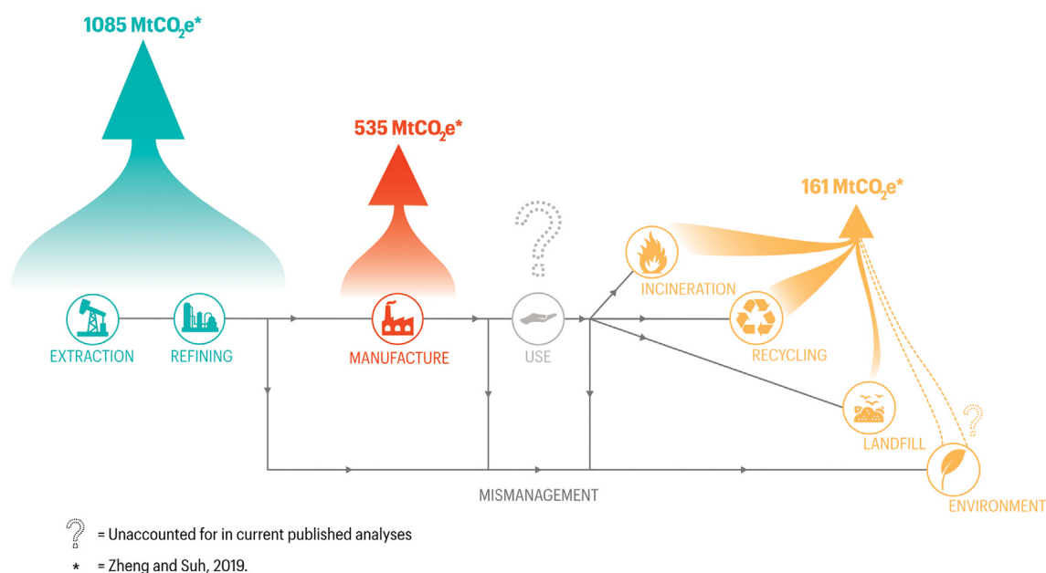
Fig. 1. The Plastic Lifecycle. Schematic representing the estimated amounts of greenhouse gases released in CO 2 e at each stage of the plastic life cycle. The amount stored during use and released when plastic ends up in the natural environment is largely unknown. Data taken from Zheng and Suh (2019).
