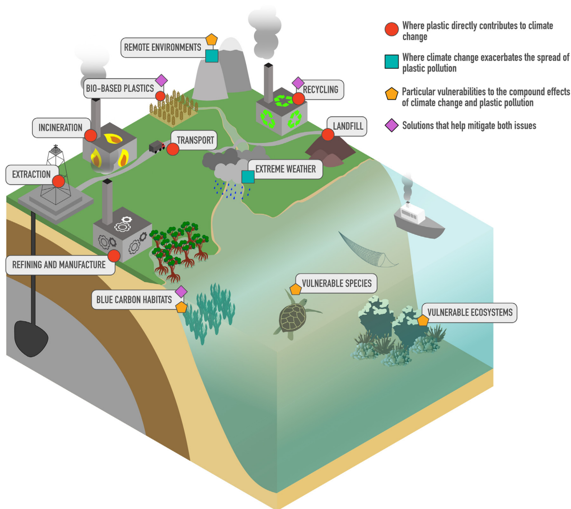
Fig. 4. Interactions between plastic and climate. A schematic illustrating points that we make throughout this article, whereby plastic will affect climate change through the contribution of GHGs and interact with the impacts of climate change in the natural environment. Coloured shapes indicate how each component is connected to both plastic pollution and climate change. The various stages of plastic production from extraction to waste management contribute to GHG emissions, while climate change can cause extreme weather events and accelerate the spread of plastics to vulnerable and remote environments. Blue carbon habitats play an important role in sequestering carbon, but they can also bury and trap plastics, preventing further spread.
