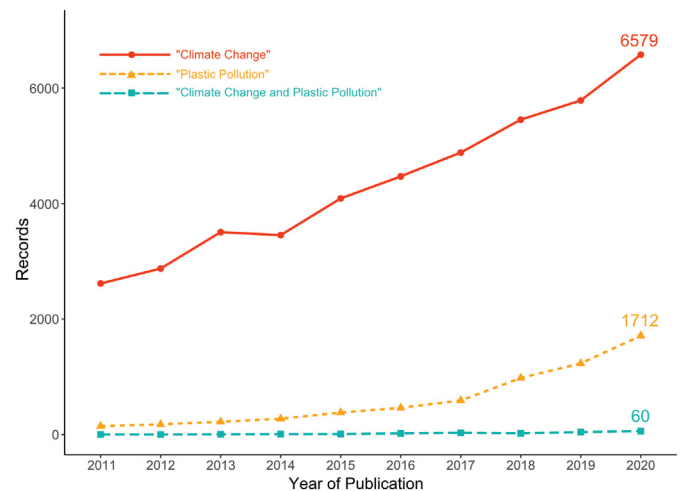
Fig. 3. Web of Science search results. The number of records published in the years 2011–2020 that address climate change in marine systems (top), marine plastic pollution (middle) and both plastic pollution and climate change in marine systems (bottom).
