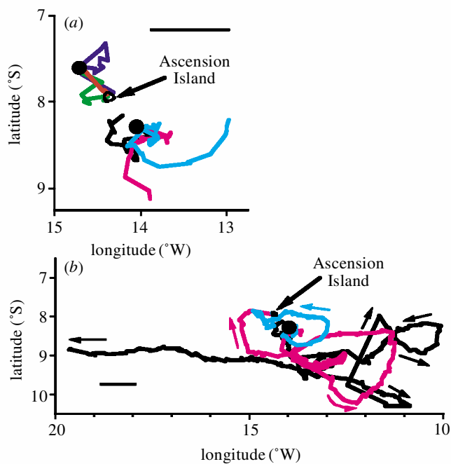
Figure 2. (a) Between 21 and 26 January 2002 the tracks of three turtles displaced by ship northwest (downwind) of Ascension Island and three turtles displaced southeast (upwind). After 4 days, all three turtles displaced downwind had returned to Ascension Island, but none of the three turtles displaced upwind had returned. Black circles show release points and arrows show direction of travel. (b) The complete tracks of the three turtles displaced upwind. One of these turtles (black line) had still failed to locate Ascension Island after 59 days of tracking (when transmissions ceased). Scale bars, 100 km. The differently coloured lines represent the different turtles' tracks.
