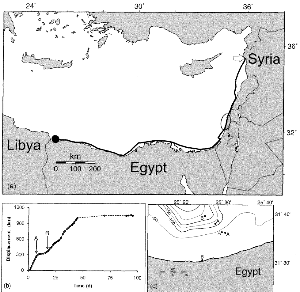
Fig. 2. (a) Migration route of a Green Turtle from nesting area in Syria to its foraging ground in Egypt. Arrow indicates start position; open oval indicates location of reduced migratory speed and a probable foraging site. Filled circle indicates end-point of the migration and location of the turtle for at least the final 26 days of transmitter activity. (b) Displacement plot indicating open sea (left of arrow labelled A) and coastal movements and presumed foraging activity (between arrows A and B). Slope of line is indicative of speed. (c) Turtle locations obtained from the foraging ground at end of migration and transmitter activity. Lines and numbers are isobaths in metres.
